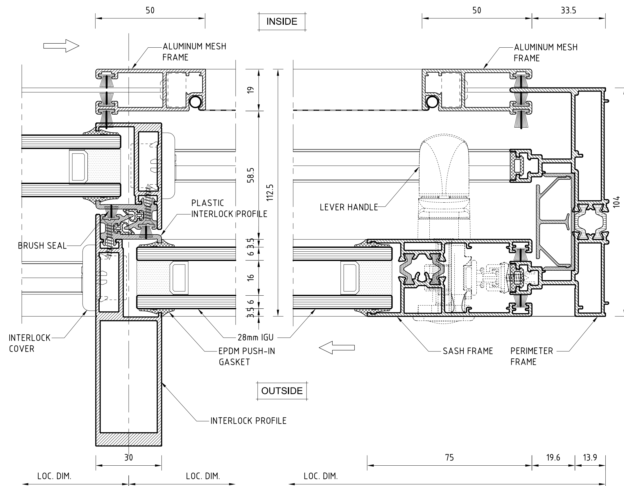
INTERLOCK DETAIL
