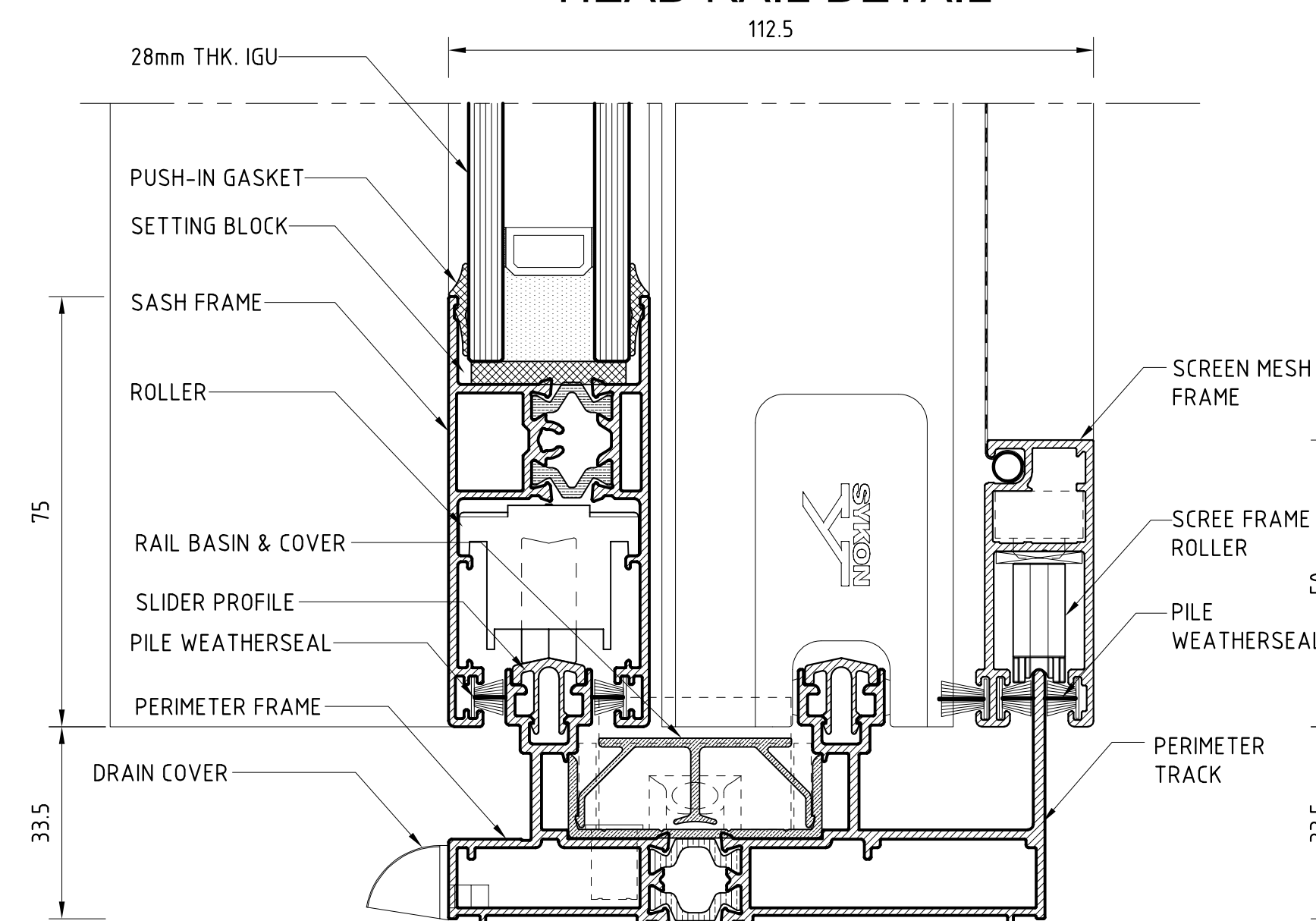
HEAD RAIL DETAIL
